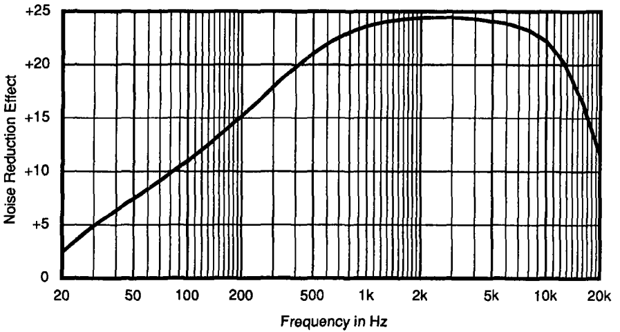
Fig.18 Maximum Noise Reduction Effect versus Frequency
